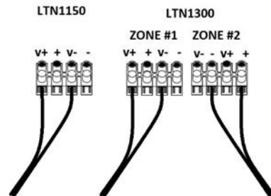
LTN1150 with single wire
