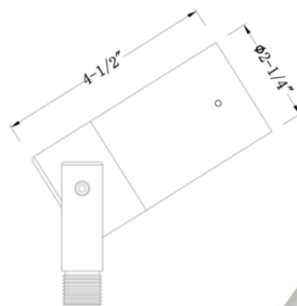
UPLIGHT ACU SERIES
